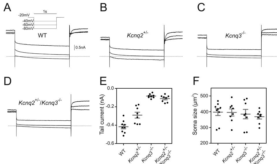
FIGURE 3. M-current in TrkB-expressing DRG neurons depends on KCNQ2 and KCNQ3. A–D, representative traces of M-current deactivation by patch clamp in cultured DRG neurons (1–2 days in vitro ) labeled with TrkB antibody from WT (9 cells) (A), Kcnq2 +/- (8 cells) (B), Kcnq3 -/- (8 cells) (C), and Kcnq2 +/- / Kcnq3 -/- (8 cells) (D) mice. E, tail current measurements at membrane voltages clamped to -40 mV. Currents were statistically significantly reduced in Kcnq2 +/- ( p = 0.0061 ), Kcnq3 -/- ( p = 0.0006 ), and Kcnq2 +/- / Kcnq3 -/- ( p = 0.0006 ) when compared with WT mice. F, soma sizes of cells measured in E. Cells were hyperpolarized for 1 s from a holding potential of -20 mV (see clamp protocol in A). Dotted line denotes 0 nA. Data are reported as mean (long bar) \pm S.E. (short bars). Mann-Whitney U test was used to assess statistical significance.
